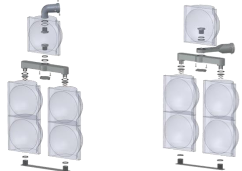
MAT-5 SEC Cluster Top Attachment
